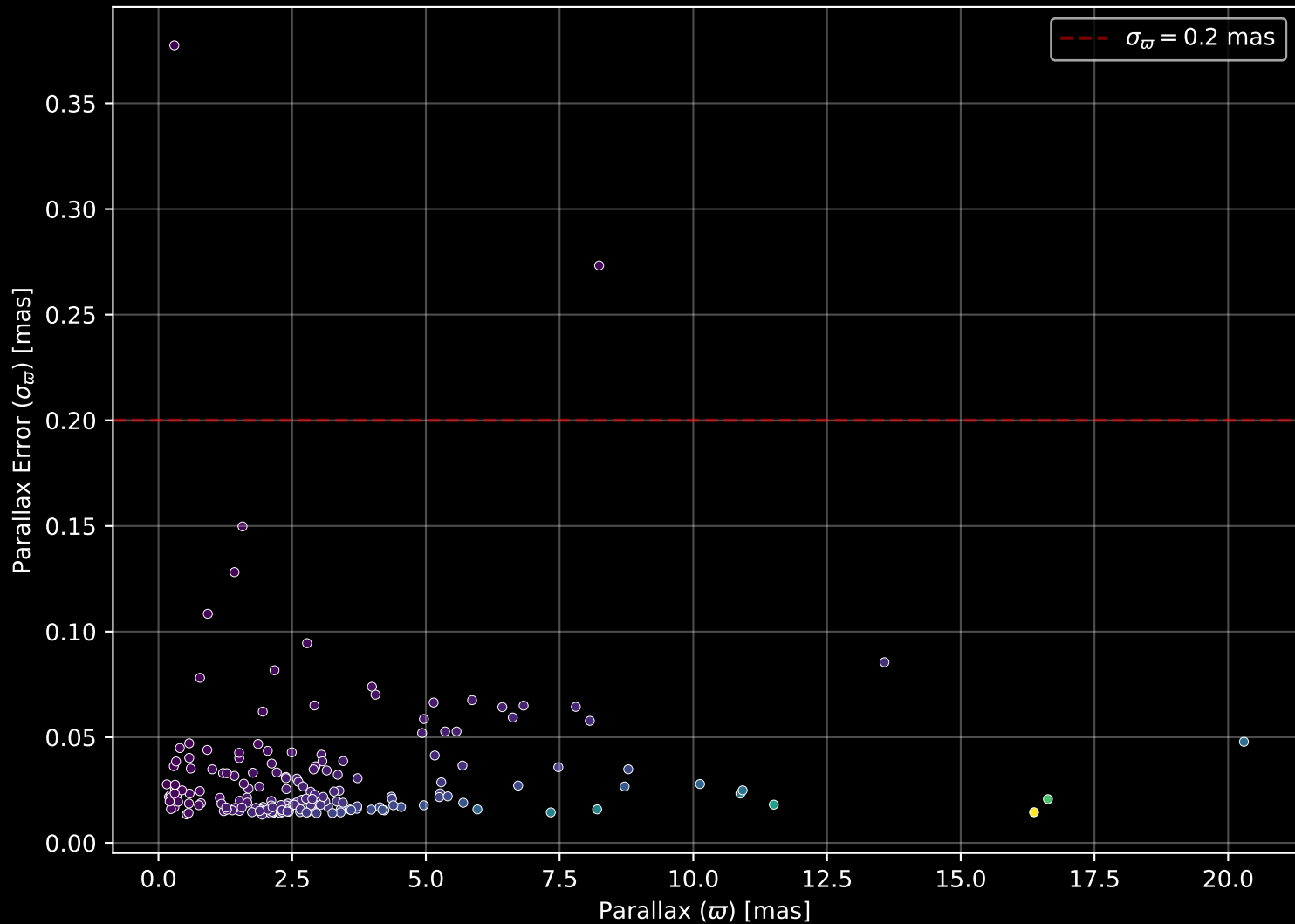
APOGEE DR17 Field: [K2_C13_185-19_btx] Parallax Quality (n= 184)
