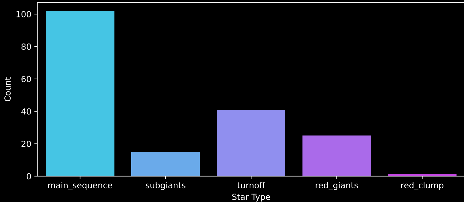
APOGEE DR17 Field: [K2_C13_185-19_btx] Count plot of Star Type
