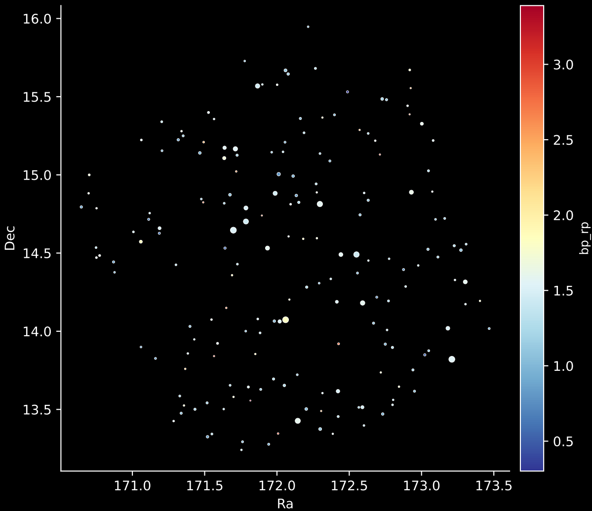
APOGEE DR17 Field: [K2_C13_185-19_btx] Stars: 184
