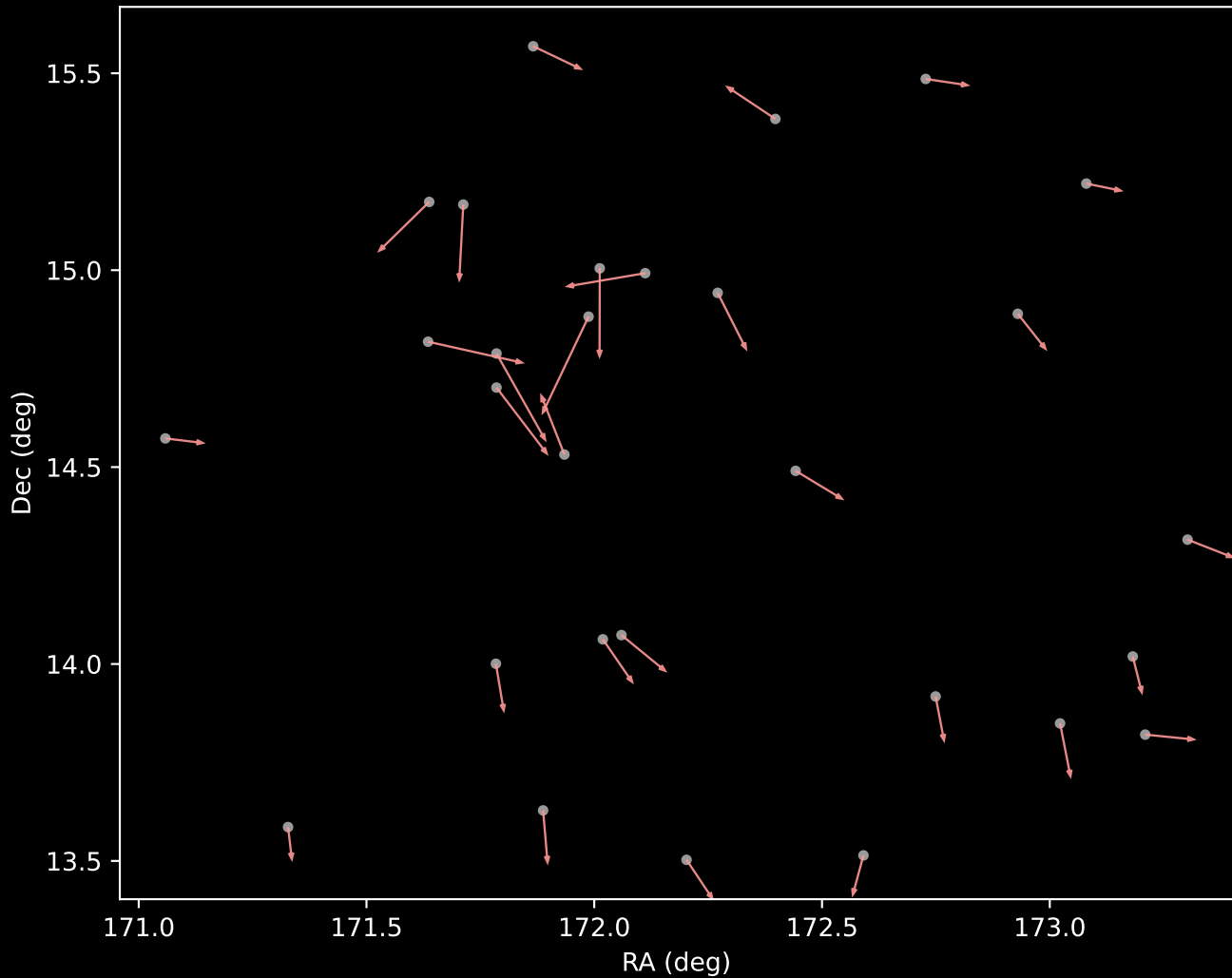
APOGEE DR17 Cluster 7 Proper Motion Vectors (n=29)
