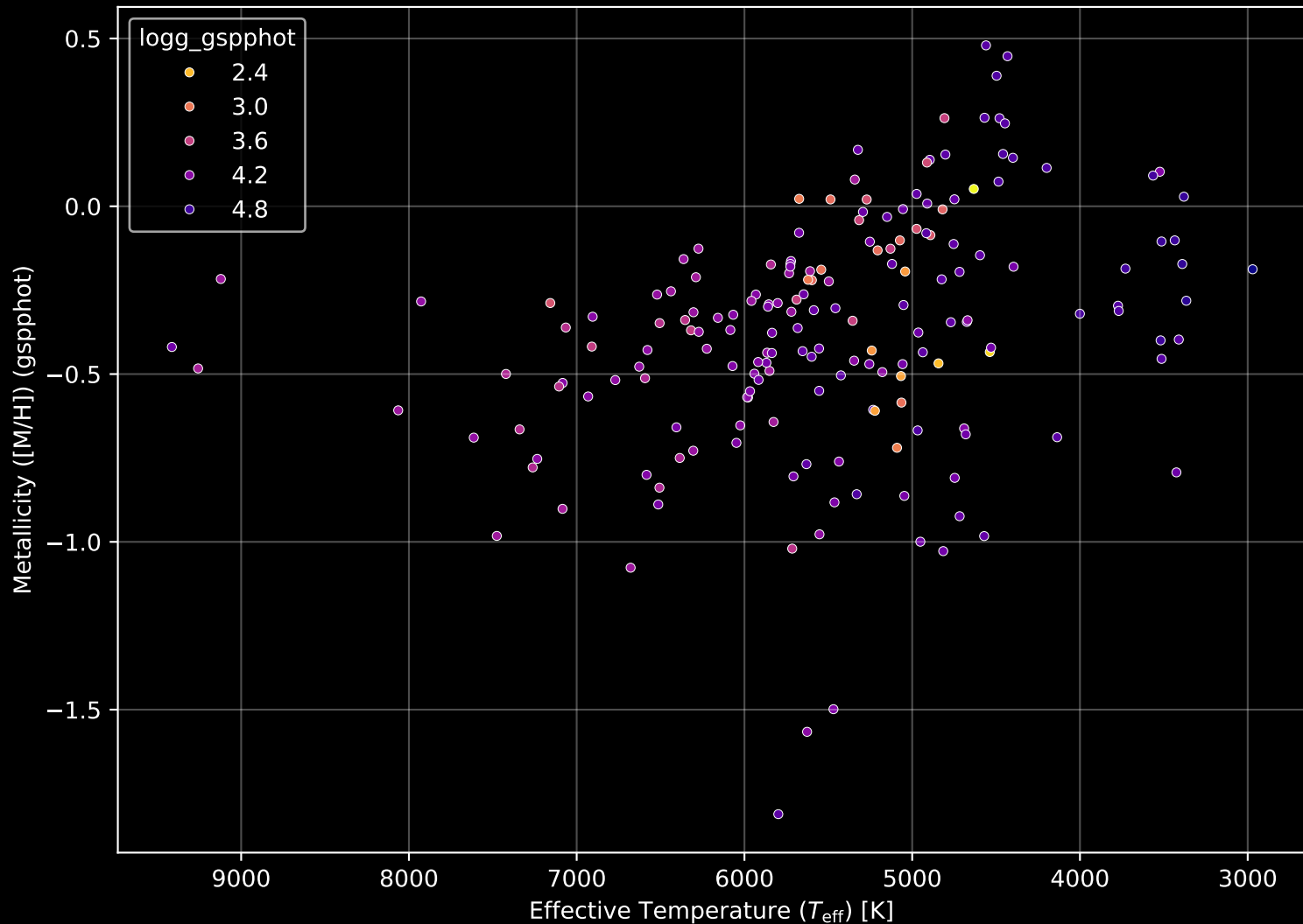
APOGEE DR17 Field: [K2_C13_185-19_btx] Stellar Population Parameters (n= 184)
