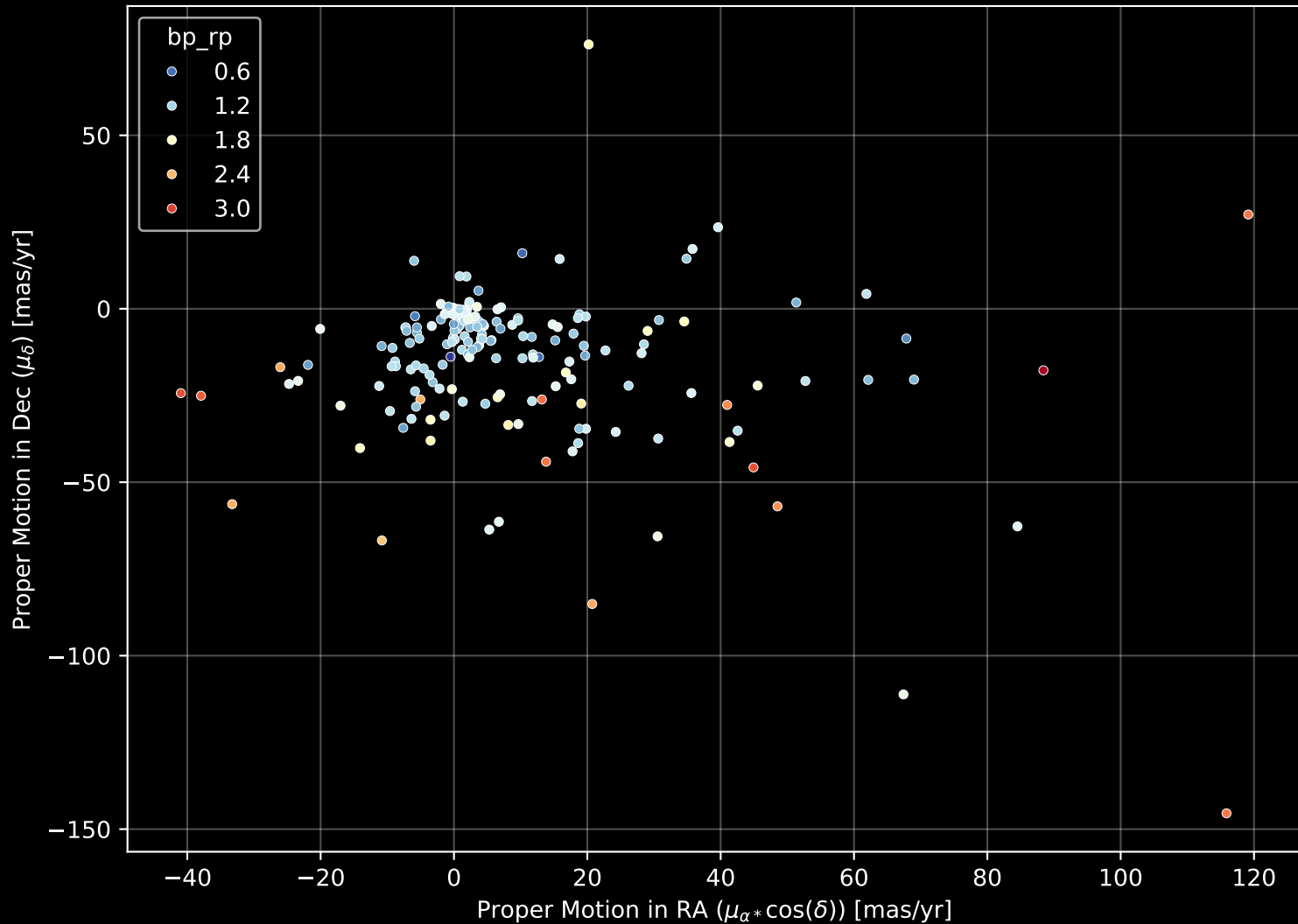
APOGEE DR17 Field: [K2_C13_185-19_btx] Proper Motion Diagram (n= 184)
