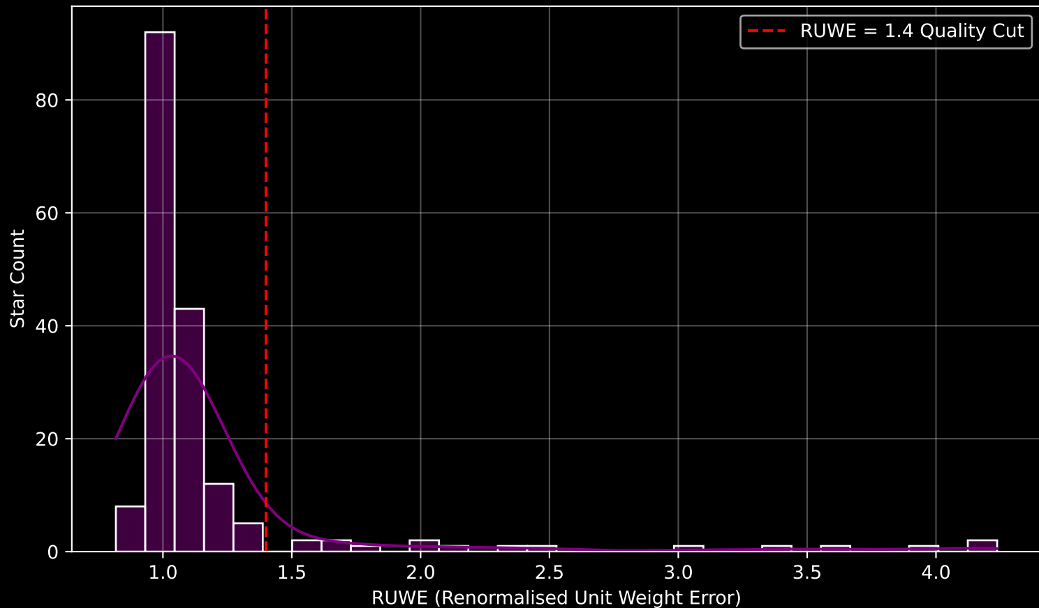
GAPOGEE DR17 Field [K2_C13_185-19_btx] RUWE Distribution (n= 176)
