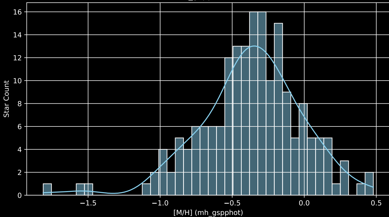
APOGEE DR17 Field: [K2_C13_185-19_btx [M/H] (mh_gspphot) (n= 184)
